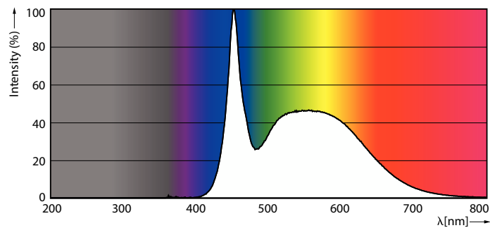
Spectral Power Distribution Colour - TForce Core HB 50W E27 865 WV G3
