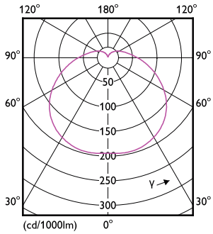
Light Distribution Diagram - TForce Core HB 50W E27 865 WV G3
