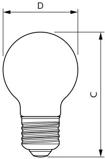
LEDClassic 4.5W G16.5 E27 827 CLND1PF/10
