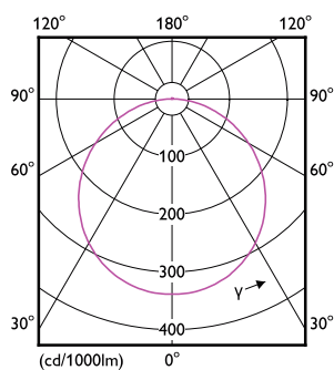
Downlight DL252 G2 LED SF RD 1300lm 40K-LDD
