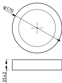
DL252 SR LED9 840 12W ?183 Latam ND
