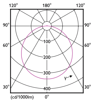
Downlight DL252 G2 LED SF RD 900lm 40K-LDD
