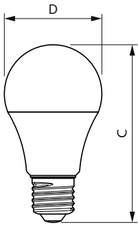
Standard LEDBulb 9W E27 3000K W 1PF/40 BR
