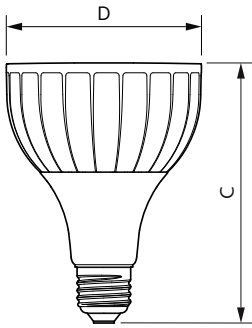
Master LED PAR30L 28W 30D 840 100-277V
