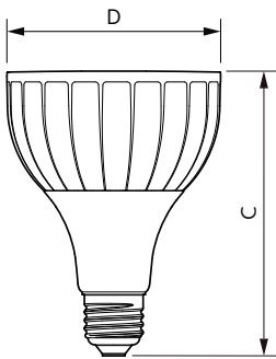
PAR30L 30-70W 3000lm 15D 3000K E27 ND
