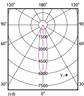
Light Distribution Diagram - PAR38 14-120W 830 25D 120V G ULW Dim E27
