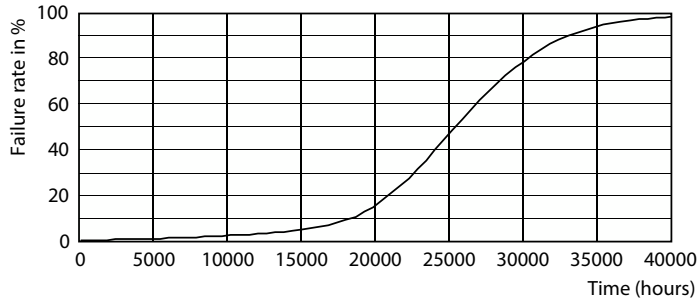
Life Expectancy Diagram - PAR38 14-120W 830 25D 120V G ULW Dim E27
