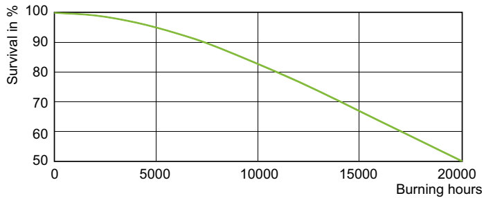
Life Expectancy Diagram - MH 400W/640 E40 CL U 1SL/6
