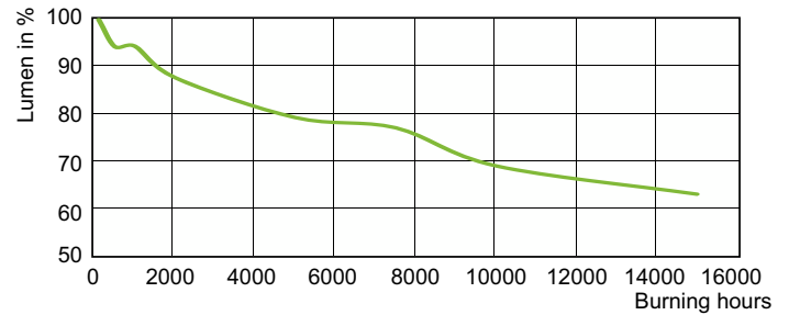
Lumen Maintenance Diagram - MH 400W/640 E40 CL U 1SL/6
