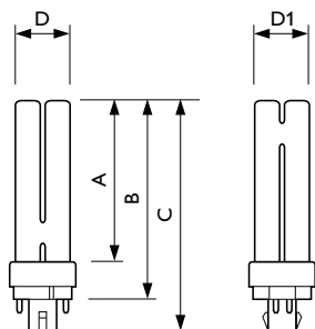
PL-C 26W/840/4P 1CT/5X10BOX
