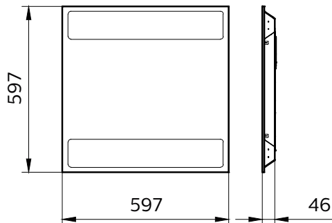
RC100X LED37S 840 W60L60 IAR OC CAU G3
